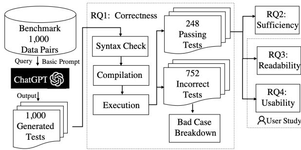
Fig. 2. The Workflow of Our Empirical Study
